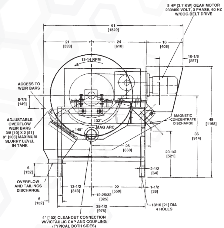
Cross-Section View - 36" Diameter Self-Leveling Separator
