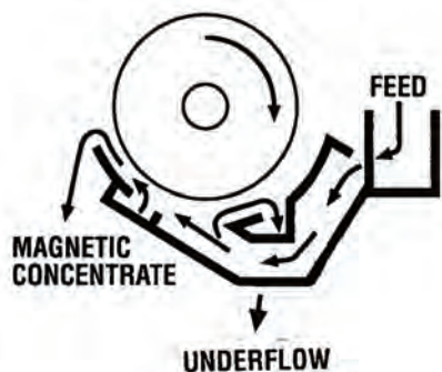
Counter-Current Tank
