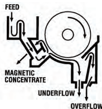
Counter-Rotation Tank
